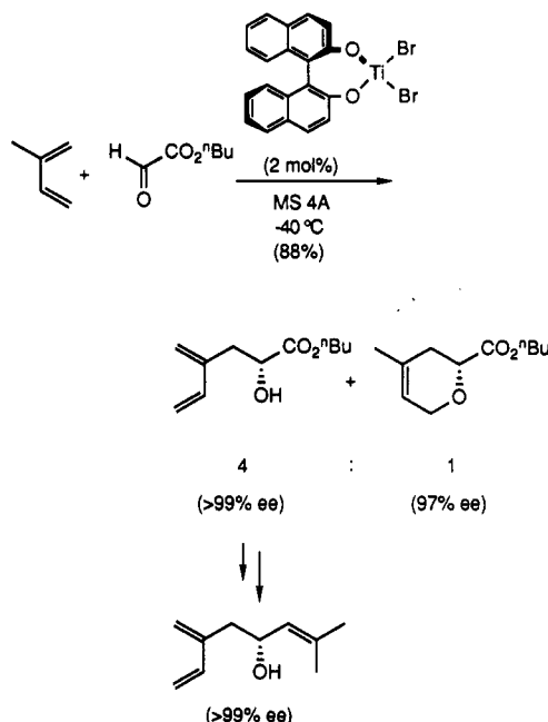
Scheme 25
