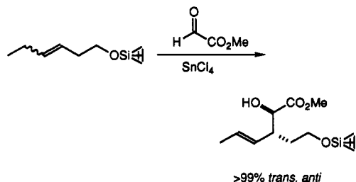
Scheme 47
