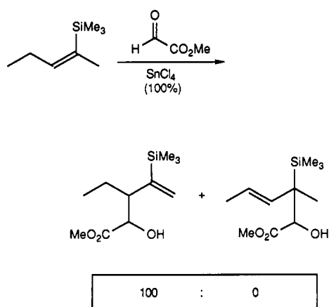
Scheme 30
