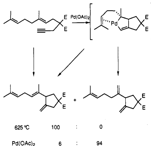
Scheme 103
