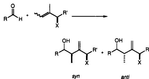
Scheme 50
