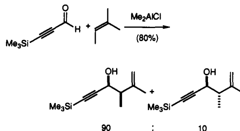
Scheme 10
