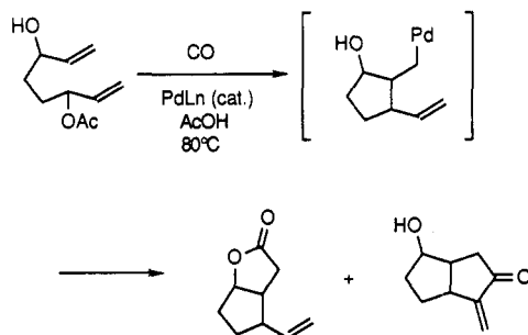
Scheme 101
