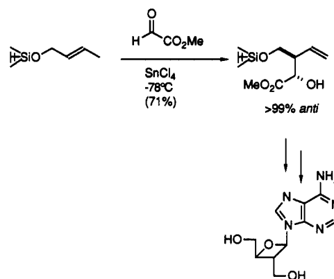
Scheme 33
