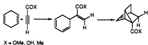
Scheme 23
