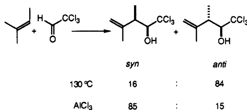
Scheme 20
