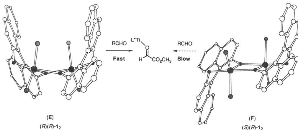
Figure 4. 3D representation of BINOL-Ti complex.
