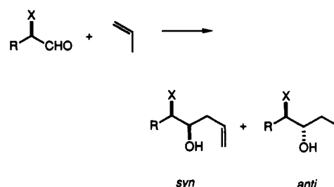
Scheme 50
