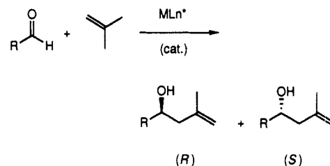
Scheme 69
