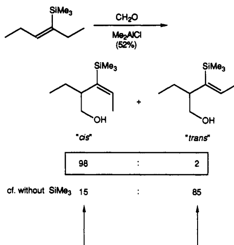
Scheme 38
