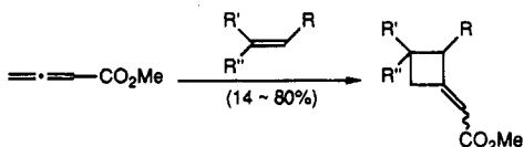
Scheme 28
