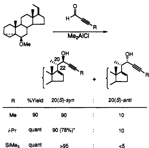
Scheme 45
