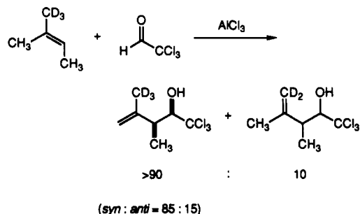
Scheme 47
