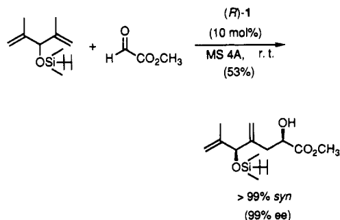
Scheme 73
