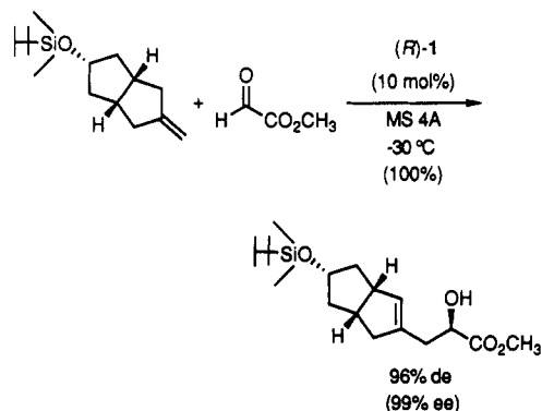
Scheme 75
