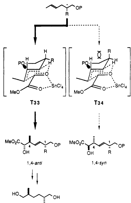
Scheme 64
