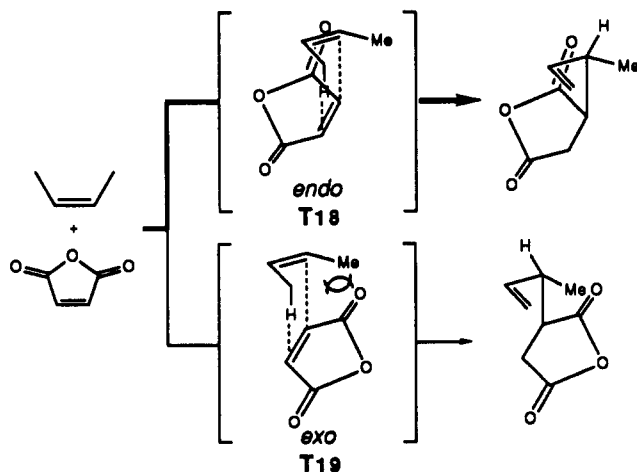
Scheme 41
