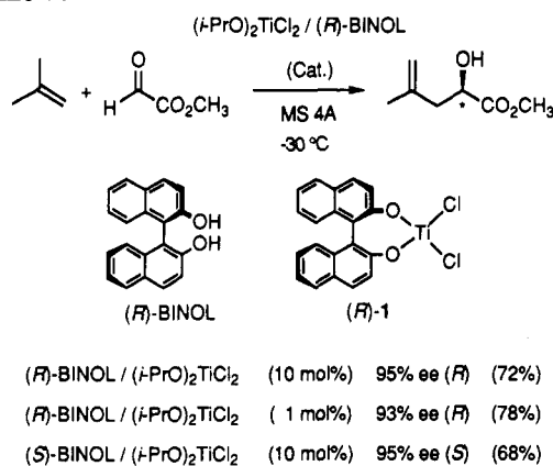
Scheme 70
