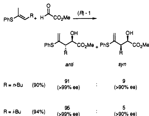
Scheme 72
