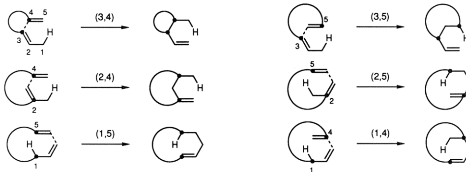
Scheme 82
