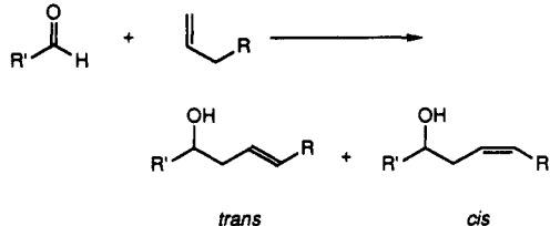
Scheme 36
