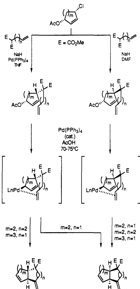
Scheme 101
