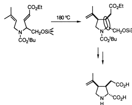
Scheme 82
