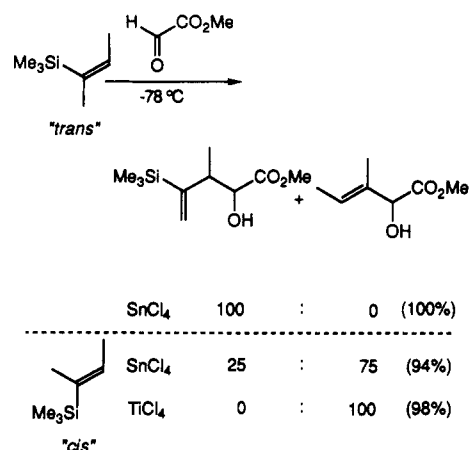
Scheme 21
