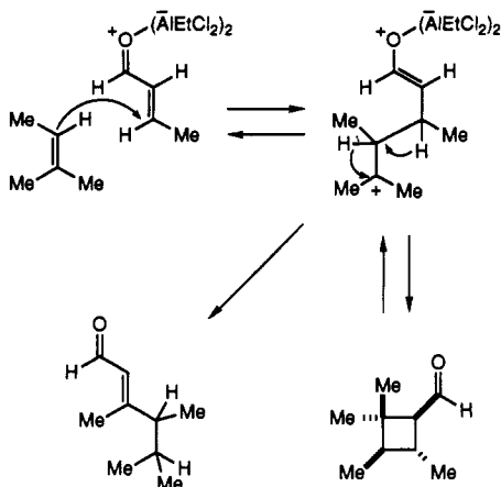
Scheme 27
