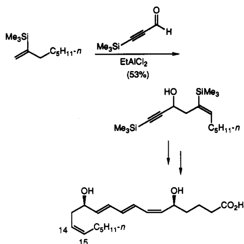
Scheme 40
