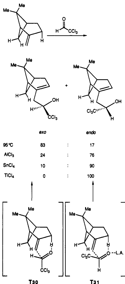
Scheme 58
