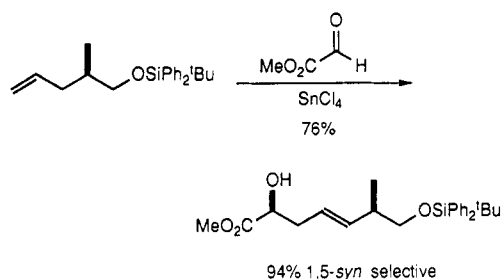
Scheme 65
