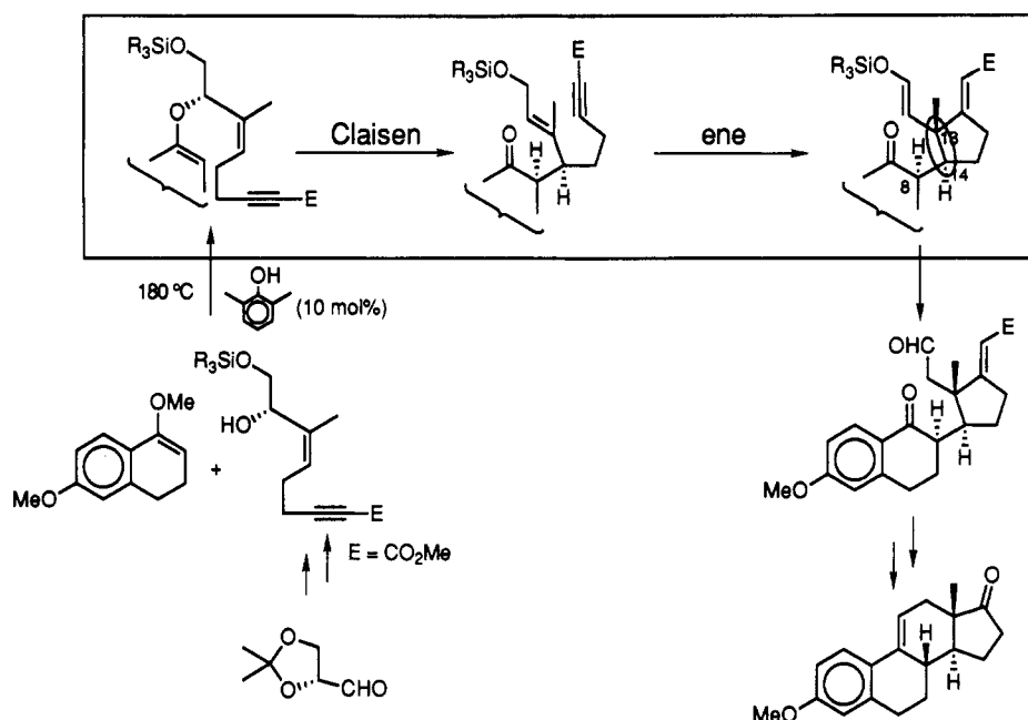
Scheme 86
