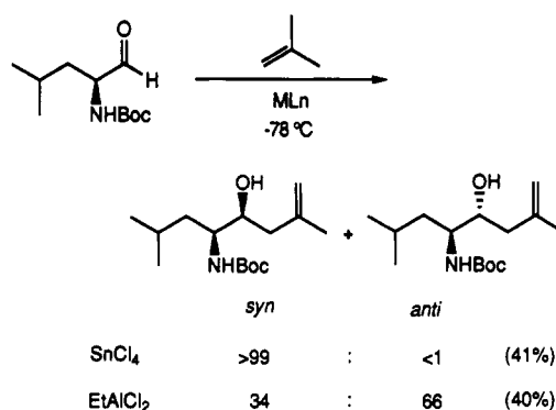
Scheme 57
