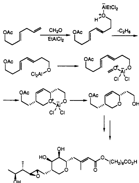
Scheme 23
