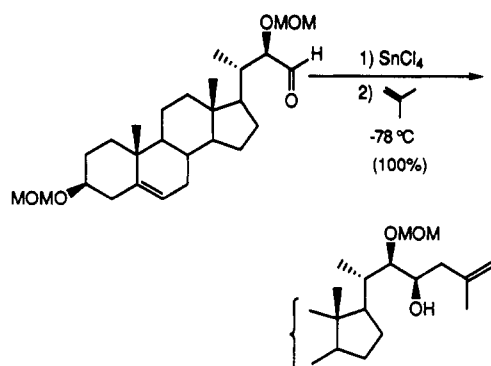
Scheme 56
