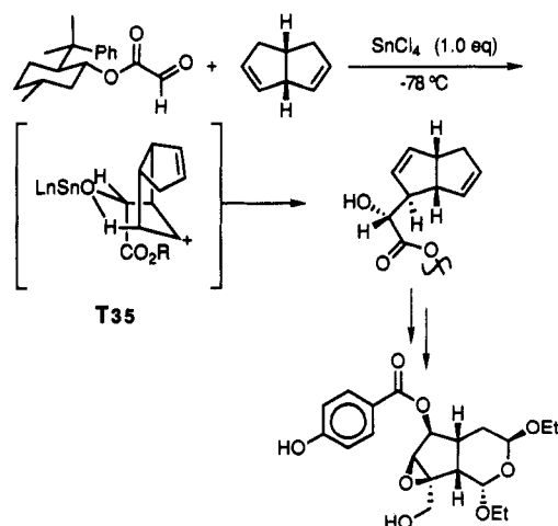
Scheme 75
