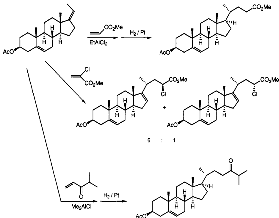
Scheme 62
