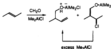
Scheme 28
