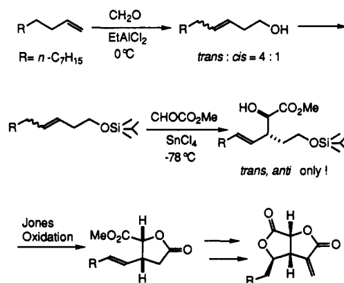
Scheme 49
