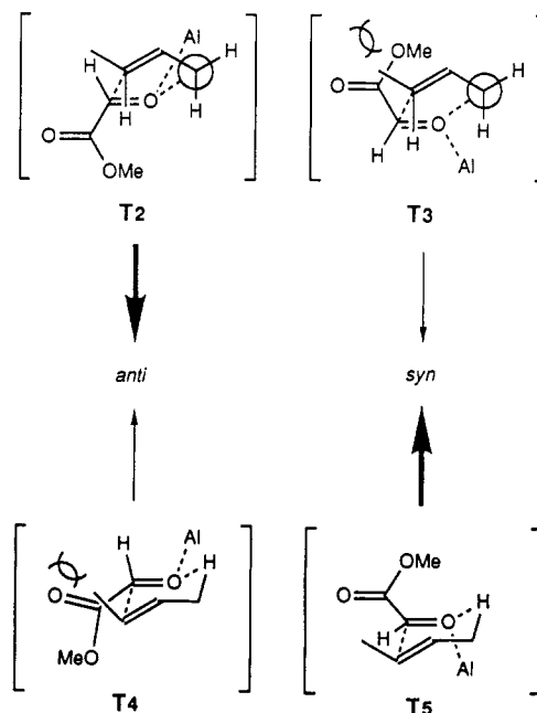
Scheme 29
