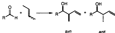
Scheme 41
