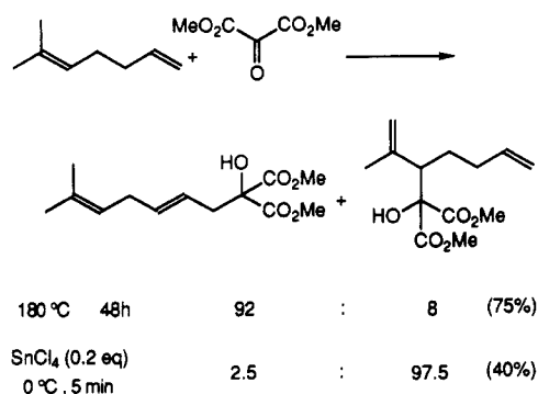
Scheme 20
