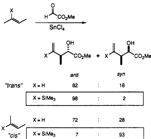
Scheme 44
