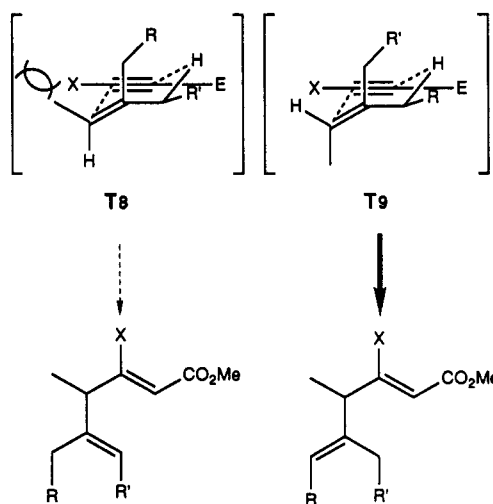
Scheme 33
