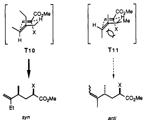
Scheme 35
